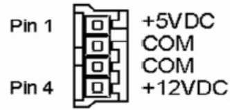
Floppy Drive Power Connector
